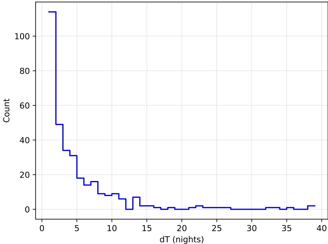
too_elab_r128_d2_giz_v3.4_10yrs all bands: DD:WFD Delta Nights Histogram
