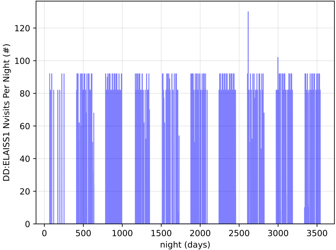
too_elab_r128_d2_giz_v3.4_10yrs all bands: DD:ELAISS1 Nvisits Per Night
