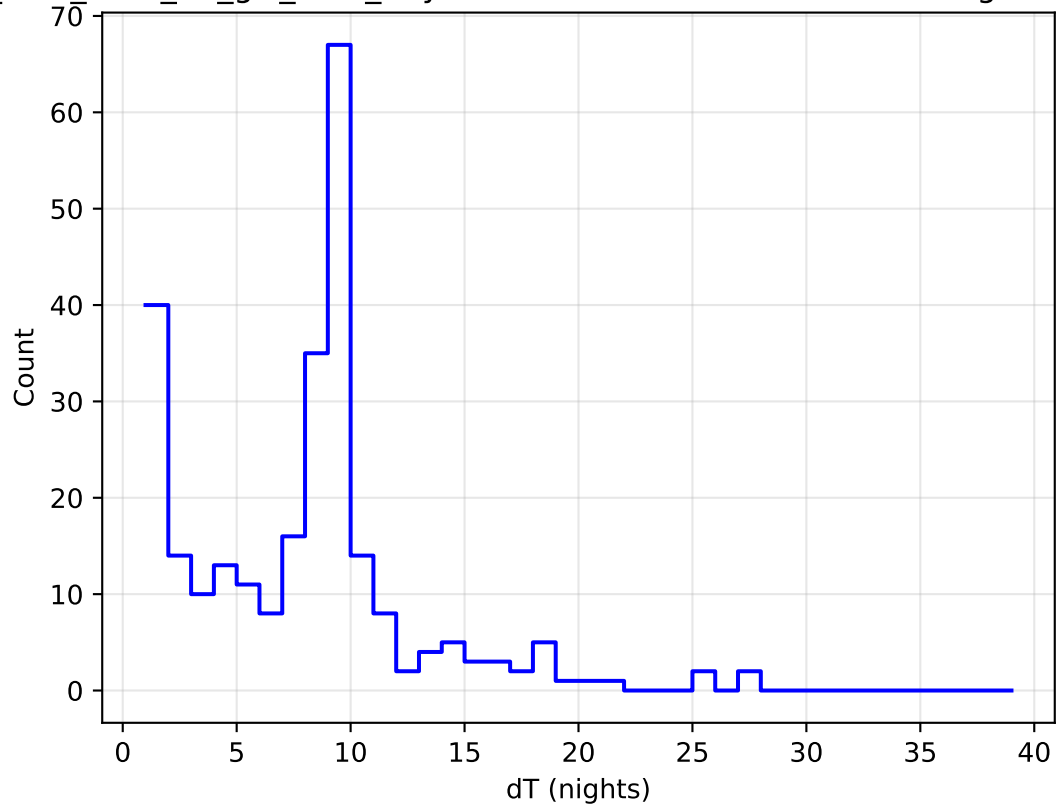
too_elab_r128_d2_giz_v3.4_10yrs all bands: DD:ELAISS1 Delta Nights Histogram
