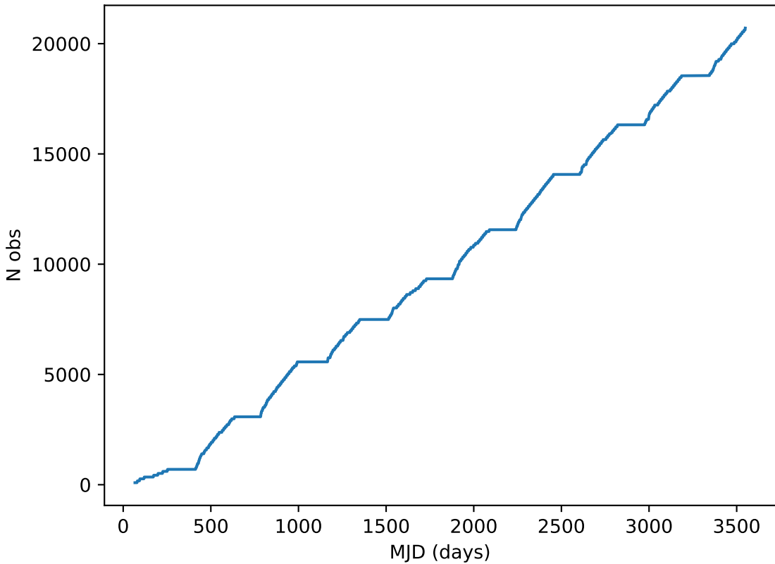
too_elab_r128_d2_giz_v3.4_10yrs all bands: DD:ELAISS1 Cumulative NVisits
