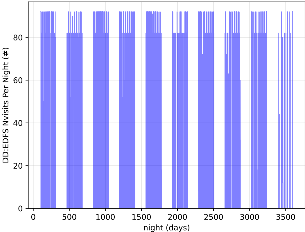
too_elab_r128_d2_giz_v3.4_10yrs all bands: DD:EDFS Nvisits Per Night
