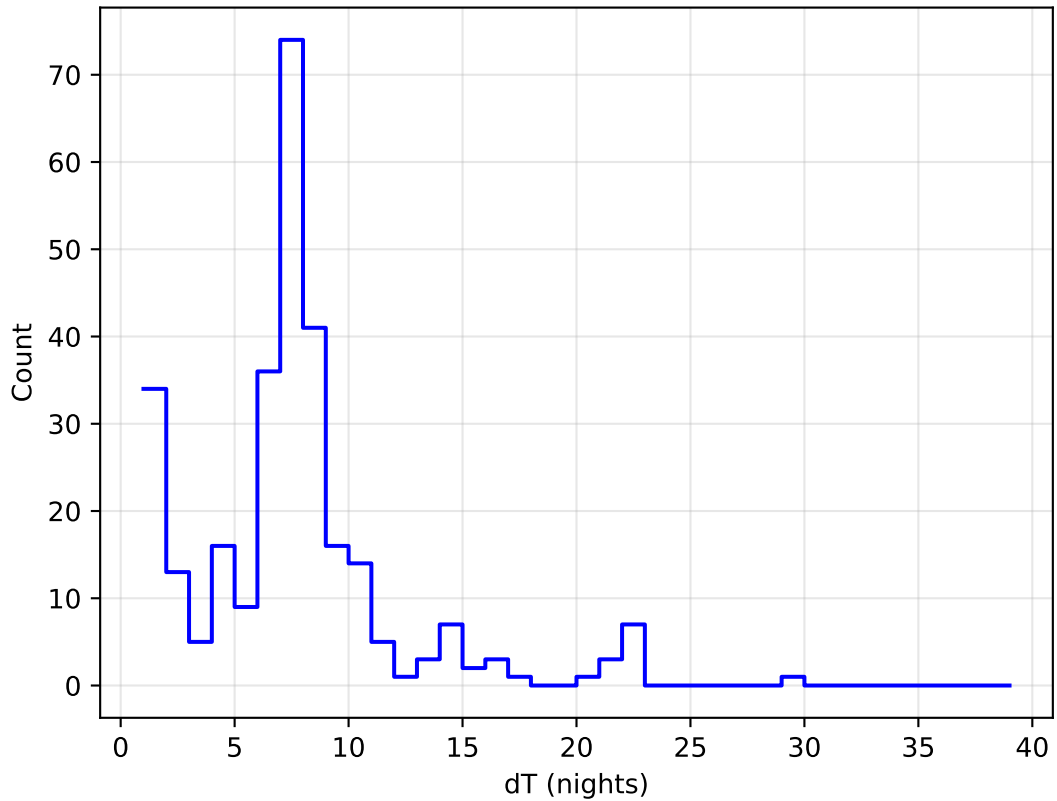
too_elab_r128_d2_giz_v3.4_10yrs all bands: DD:EDFS Delta Nights Histogram
