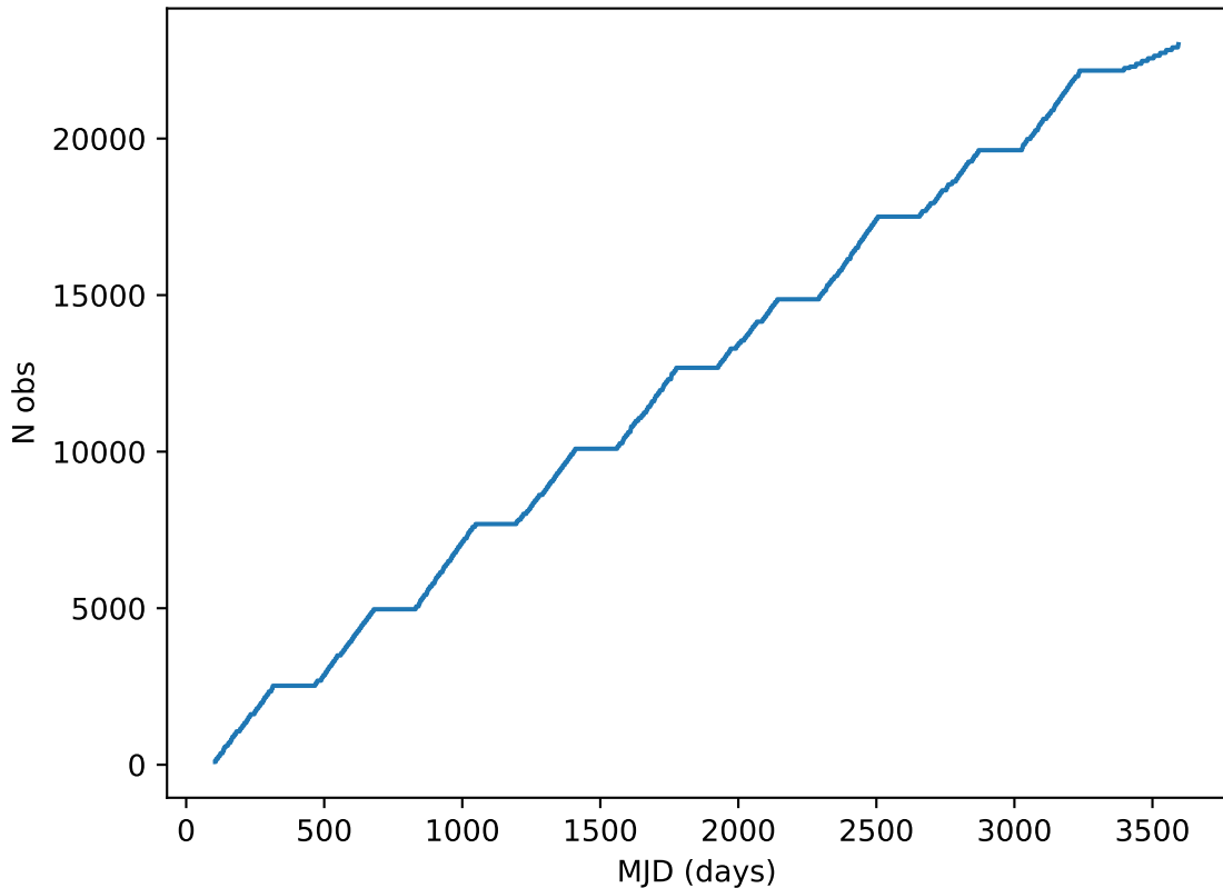
too_elab_r128_d2_giz_v3.4_10yrs all bands: DD:EDFS Cumulative NVisits
