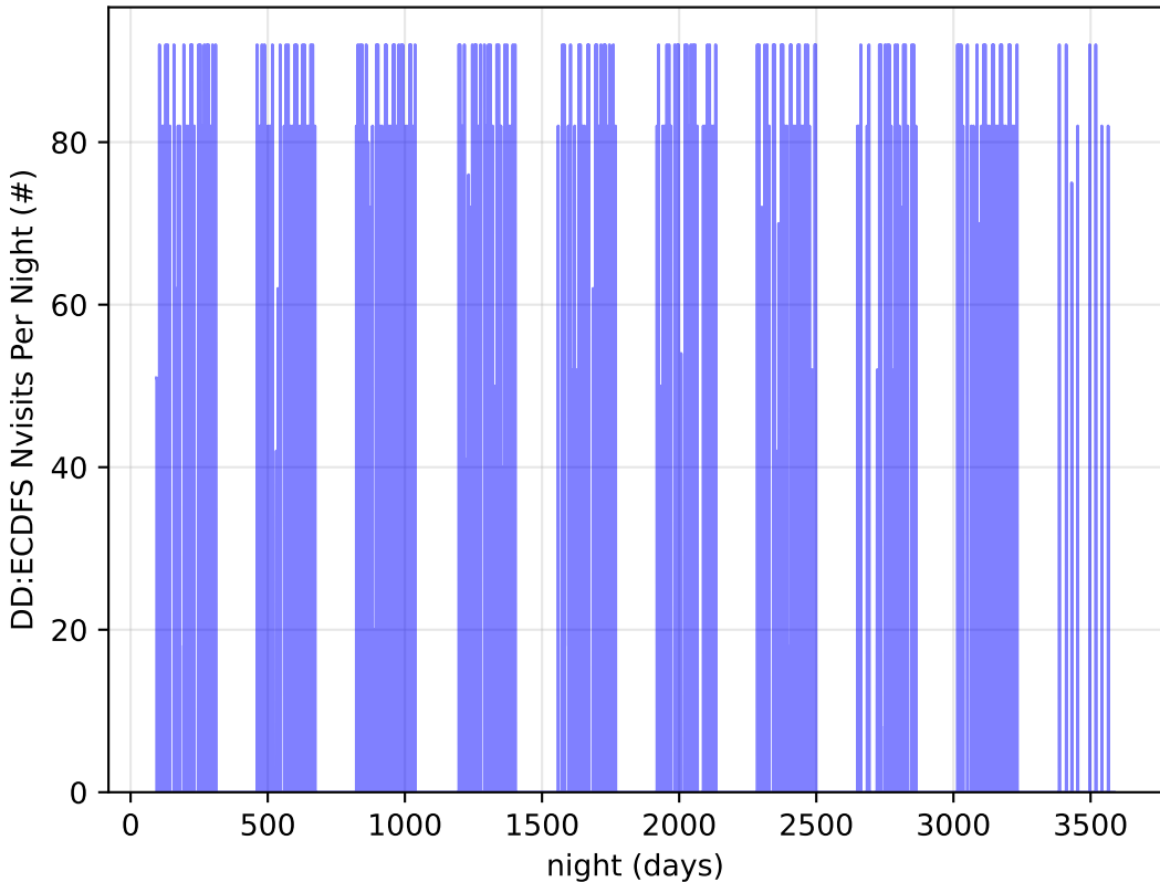
too_elab_r128_d2_giz_v3.4_10yrs all bands: DD:ECDFS Nvisits Per Night
