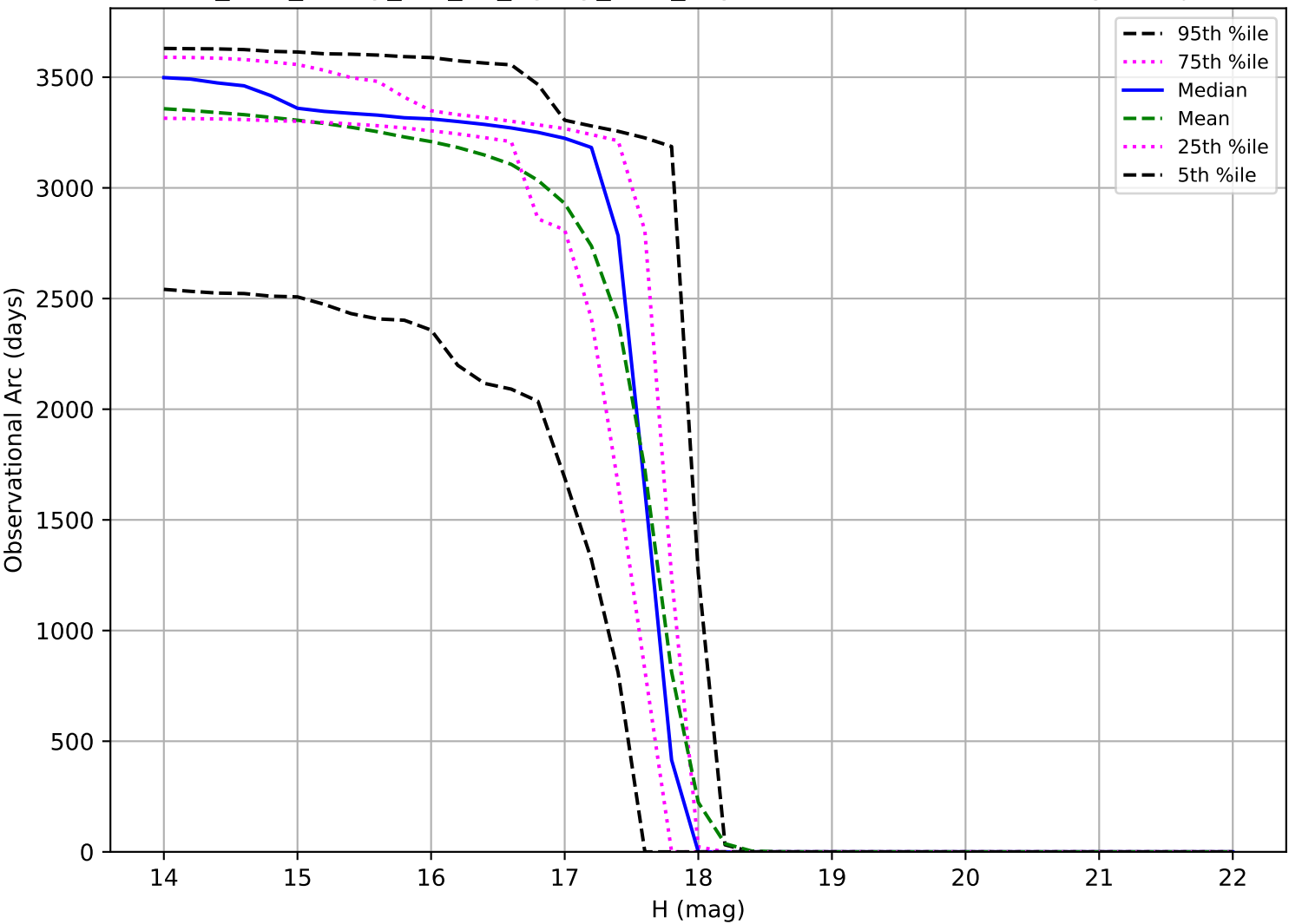
too_elab_heavy_r64_d3_ugrizy_v3.4_10yrs: Observational Arc Length Trojan
