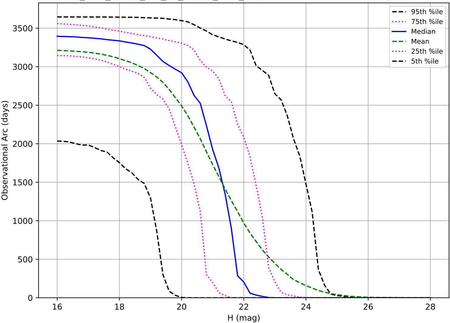
too_elab_heavy_r64_d3_ugrizy_v3.4_10yrs: Observational Arc Length PHA
