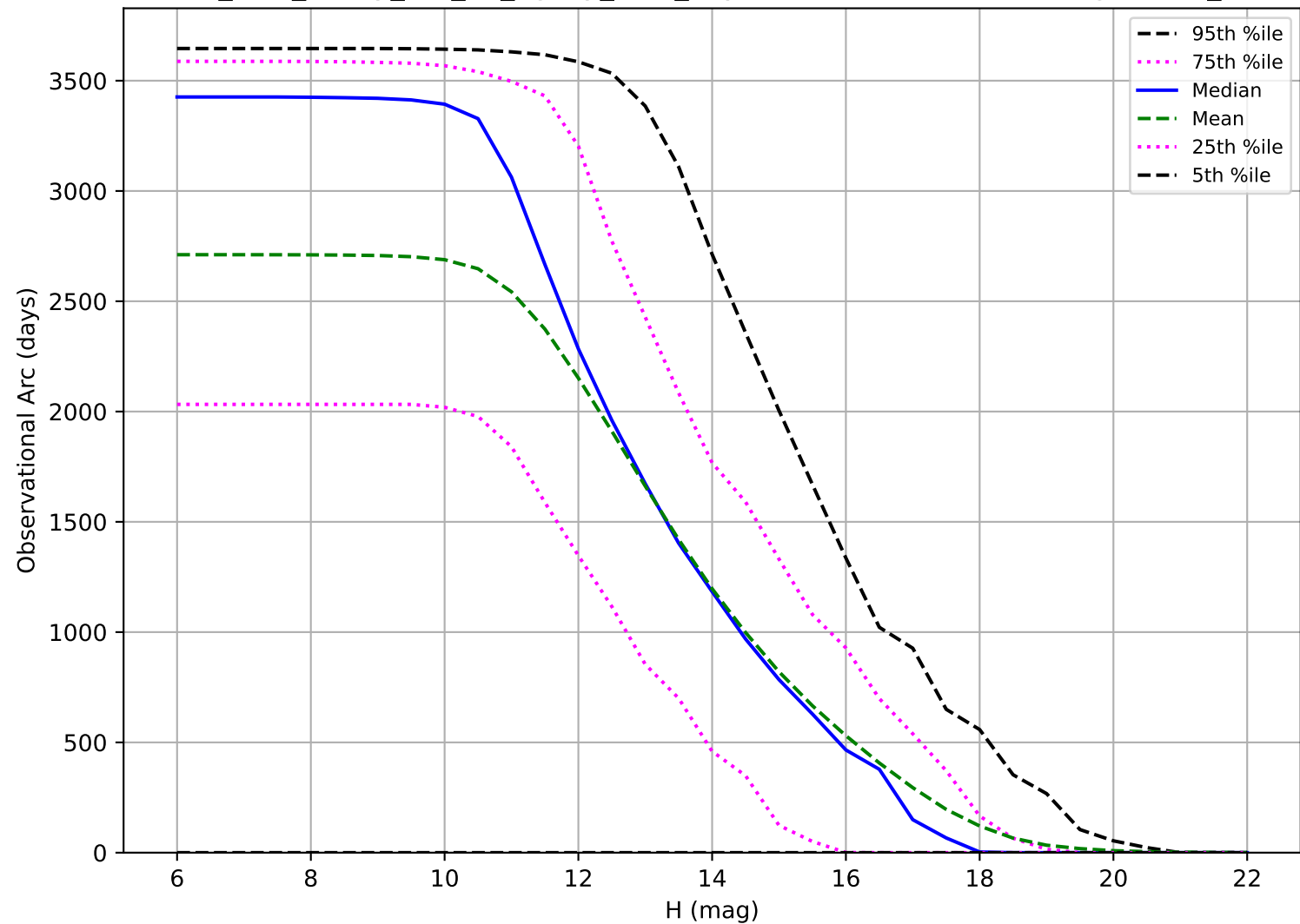
too_elab_heavy_r64_d3_ugrizy_v3.4_10yrs: Observational Arc Length OCC_r5
