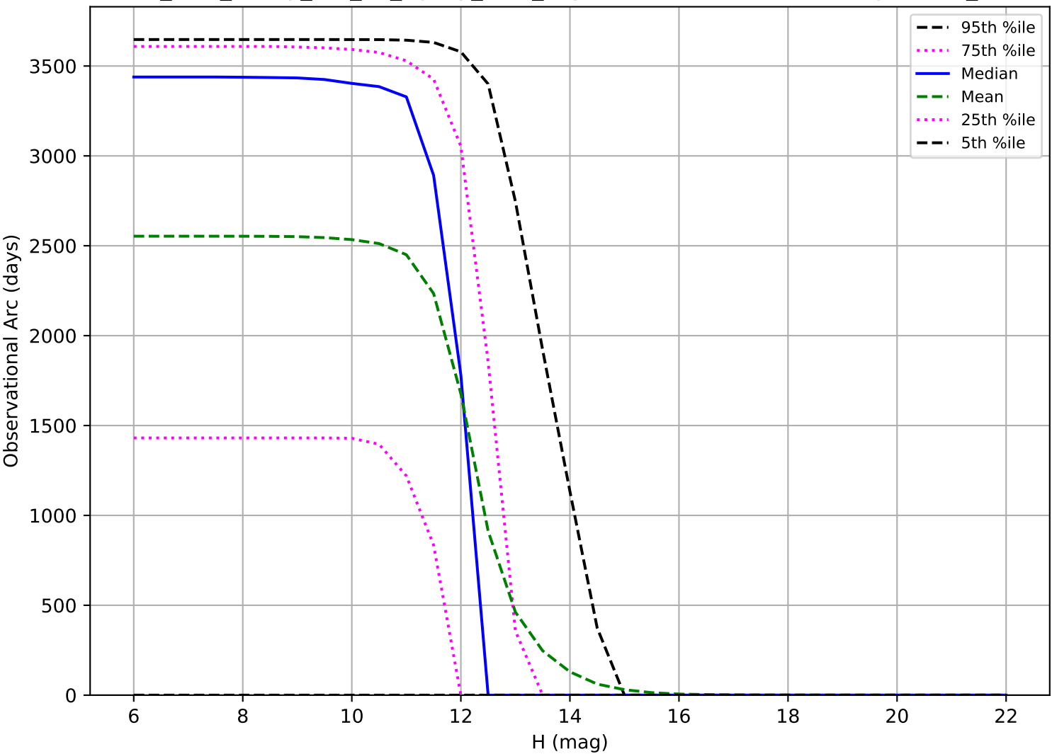
too_elab_heavy_r64_d3_ugrizy_v3.4_10yrs: Observational Arc Length OCC_r20
