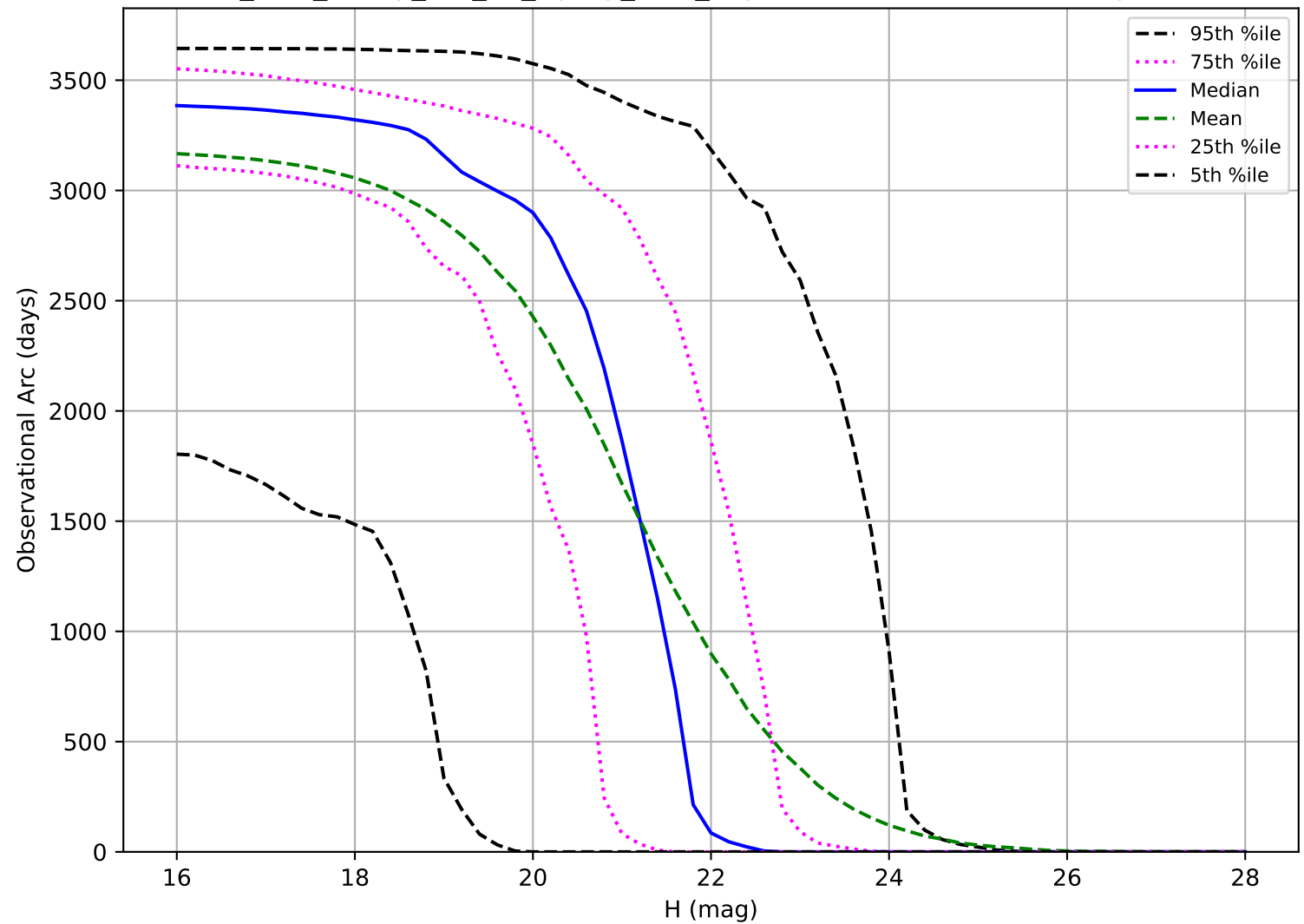
too_elab_heavy_r64_d3_ugrizy_v3.4_10yrs: Observational Arc Length NEO
