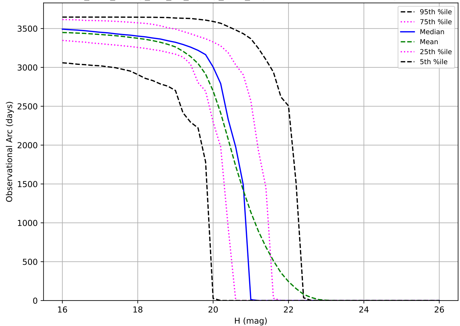
too_elab_heavy_r64_d3_ugrizy_v3.4_10yrs: Observational Arc Length MBA
