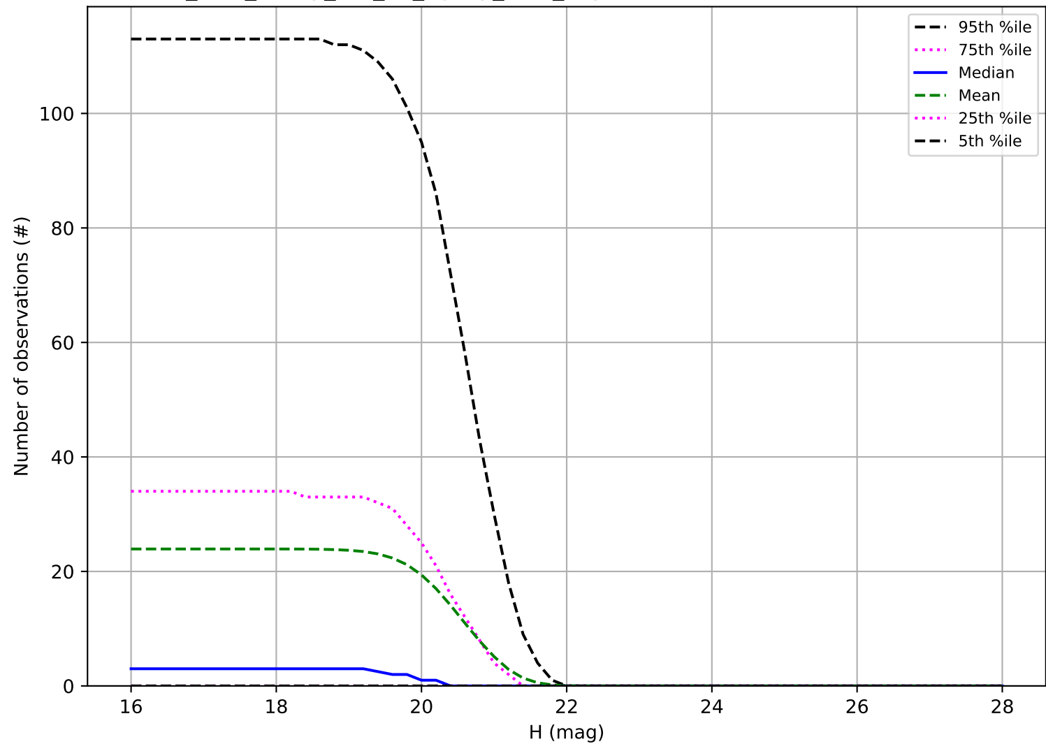
too_elab_heavy_r64_d3_ugrizy_v3.4_10yrs: Number of observations Vatira
