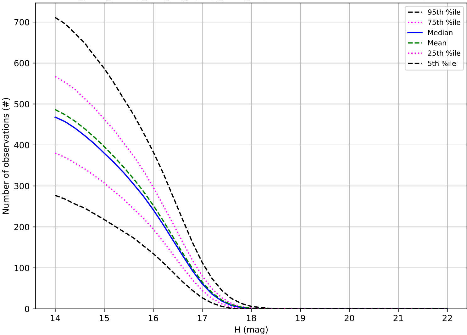
too_elab_heavy_r64_d3_ugrizy_v3.4_10yrs: Number of observations Trojan
