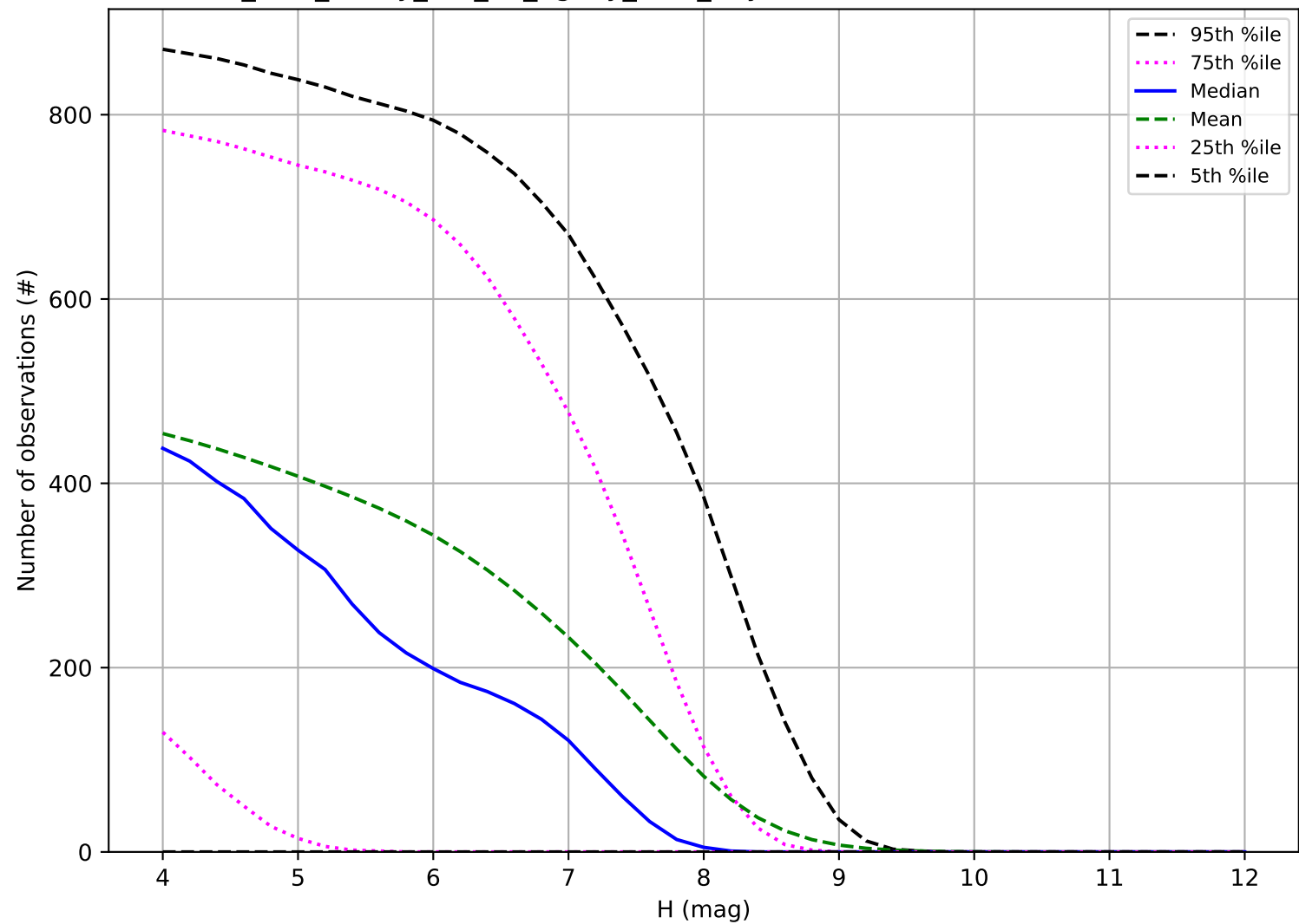
too_elab_heavy_r64_d3_ugrizy_v3.4_10yrs: Number of observations TNO
