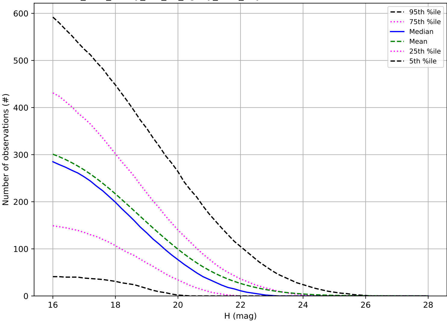
too_elab_heavy_r64_d3_ugrizy_v3.4_10yrs: Number of observations PHA
