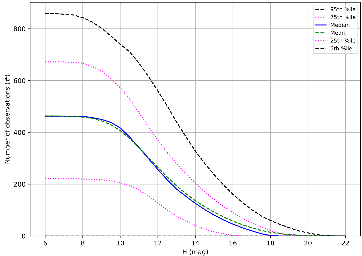
too_elab_heavy_r64_d3_ugrizy_v3.4_10yrs: Number of observations OCC_r5
