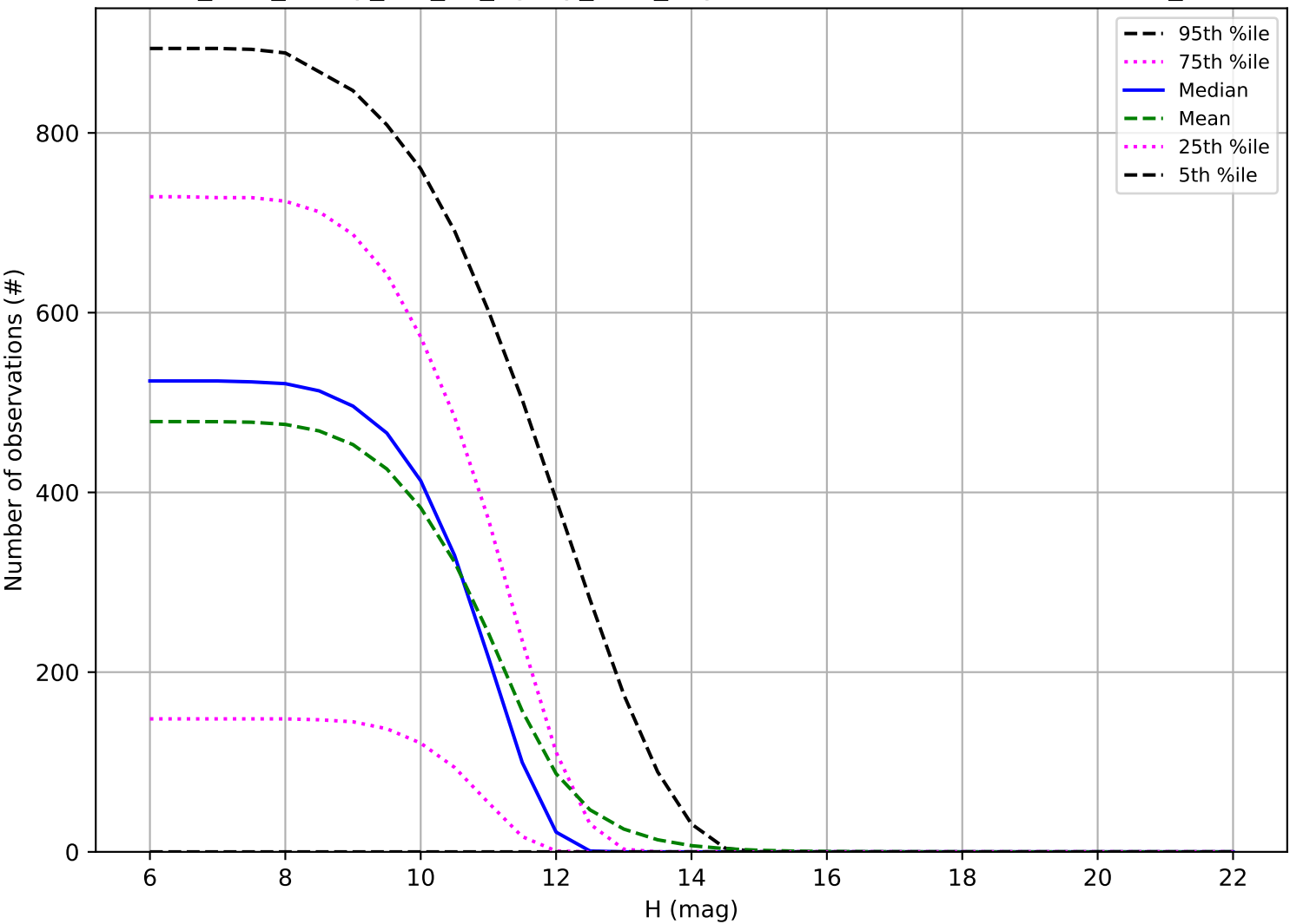
too_elab_heavy_r64_d3_ugrizy_v3.4_10yrs: Number of observations OCC_r20
