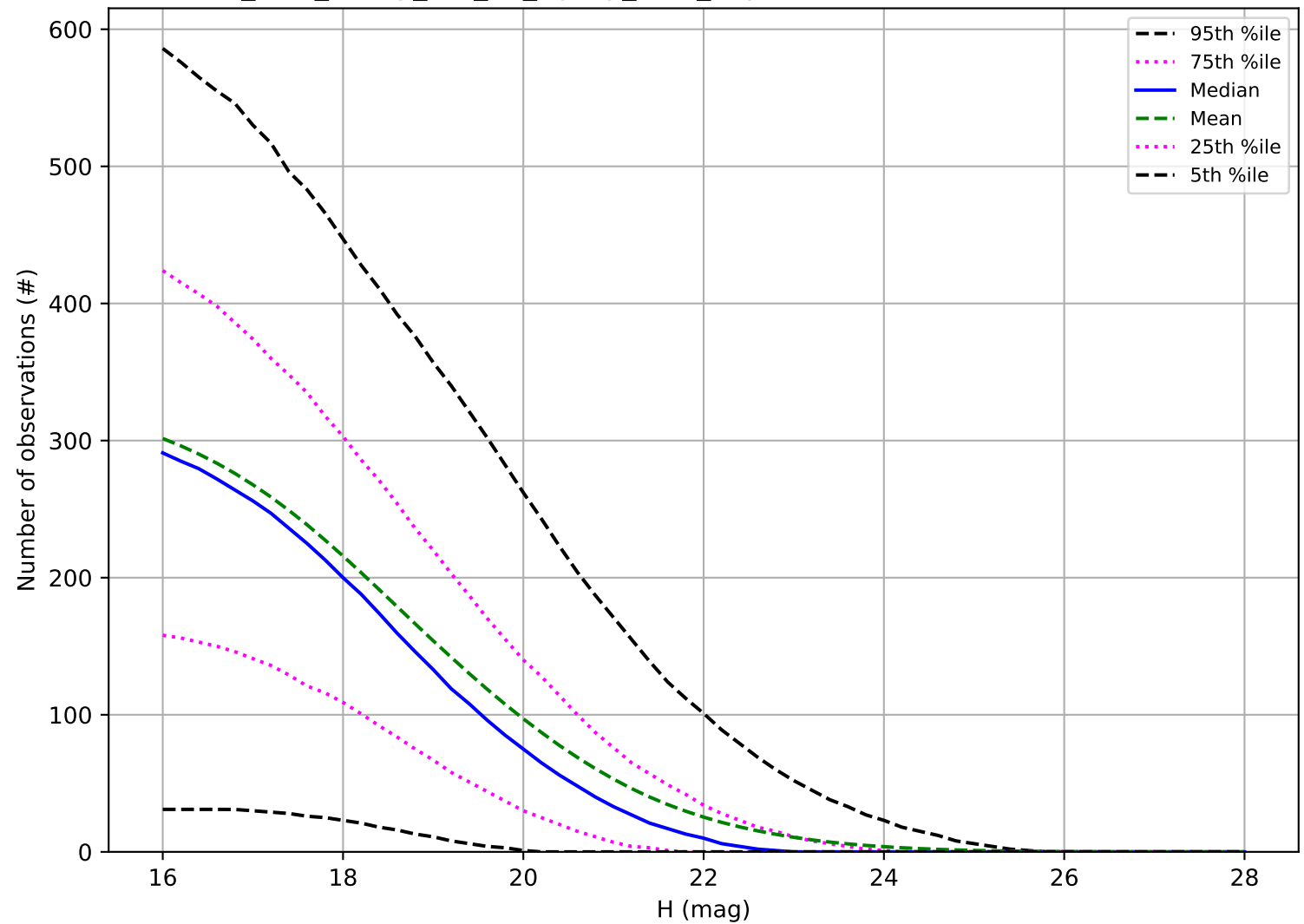
too_elab_heavy_r64_d3_ugrizy_v3.4_10yrs: Number of observations NEO
