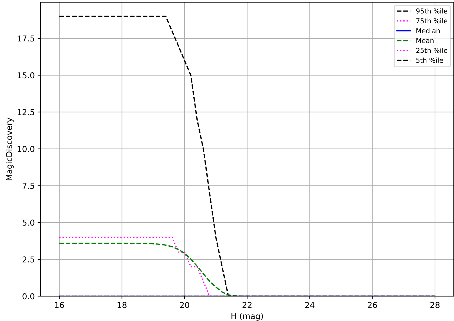
too_elab_heavy_r64_d3_ugrizy_v3.4_10yrs: Vatira 6 detections in 60 nights detection loss
