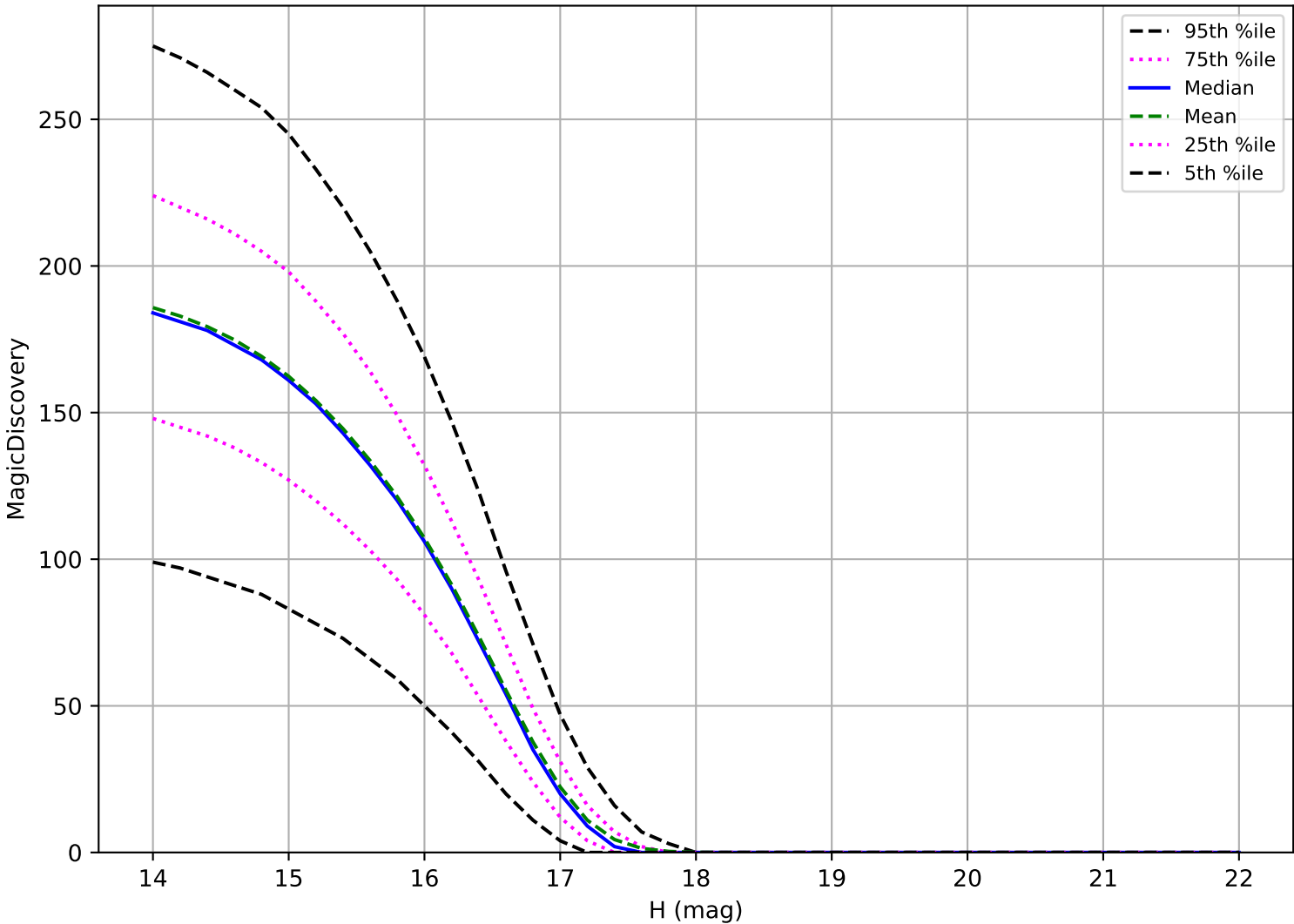
too_elab_heavy_r64_d3_ugrizy_v3.4_10yrs: Trojan 6 detections in 60 nights detection loss
