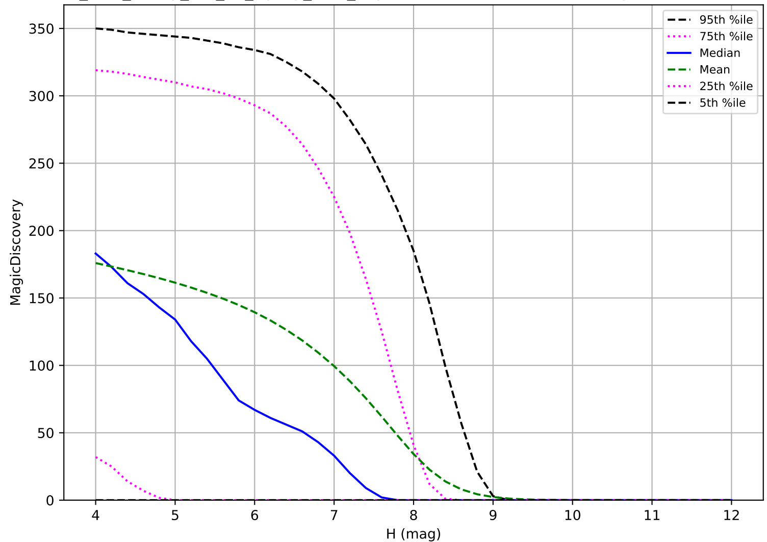
too_elab_heavy_r64_d3_ugrizy_v3.4_10yrs: TNO 6 detections in 60 nights detection loss
