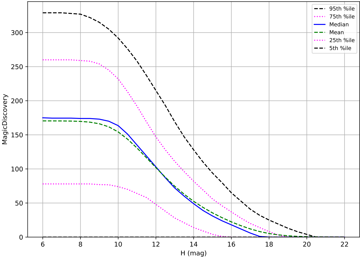
too_elab_heavy_r64_d3_ugrizy_v3.4_10yrs: OCC_r5 6 detections in 60 nights detection loss
