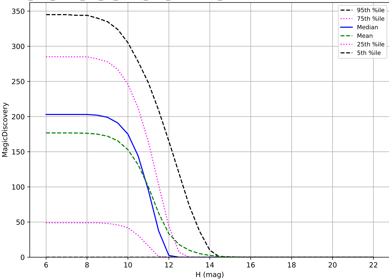
too_elab_heavy_r64_d3_ugrizy_v3.4_10yrs: OCC_r20 6 detections in 60 nights detection loss
