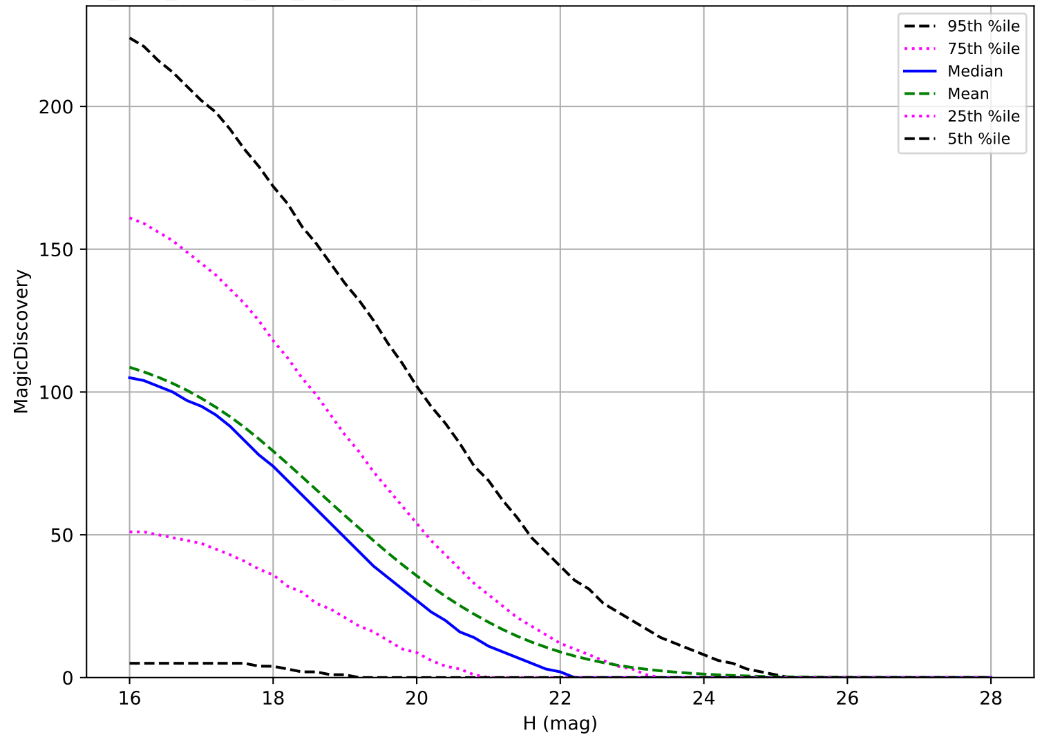
too_elab_heavy_r64_d3_ugrizy_v3.4_10yrs: NEO 6 detections in 60 nights detection loss
