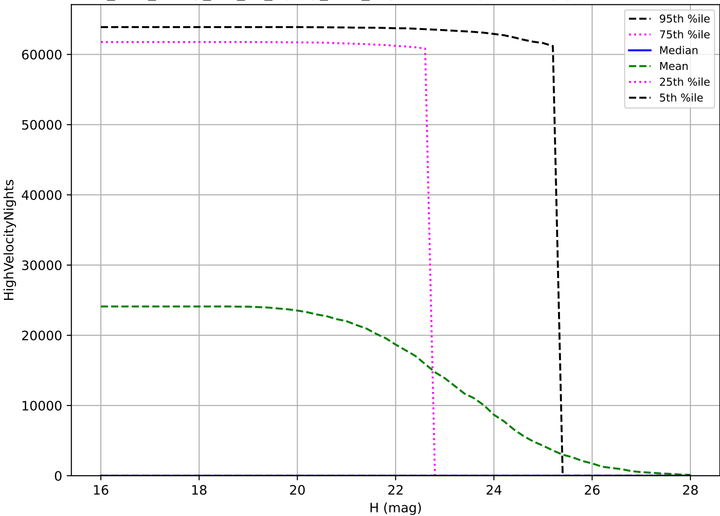
too_elab_heavy_r64_d3_ugrizy_v3.4_10yrs: PHA High velocity pair detection loss
