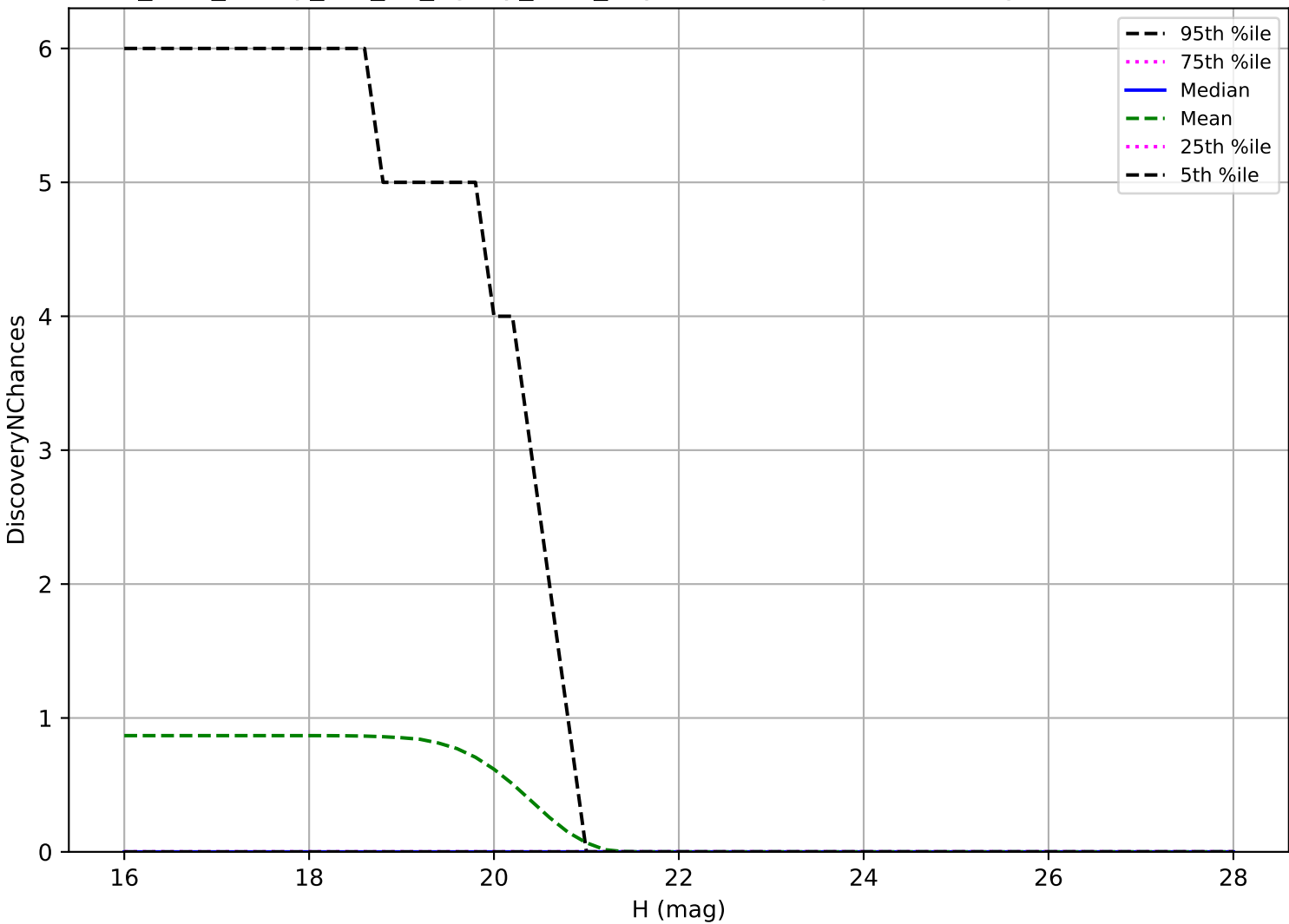
too_elab_heavy_r64_d3_ugrizy_v3.4_10yrs: Vatira 3 pairs in 15 nights detection loss
