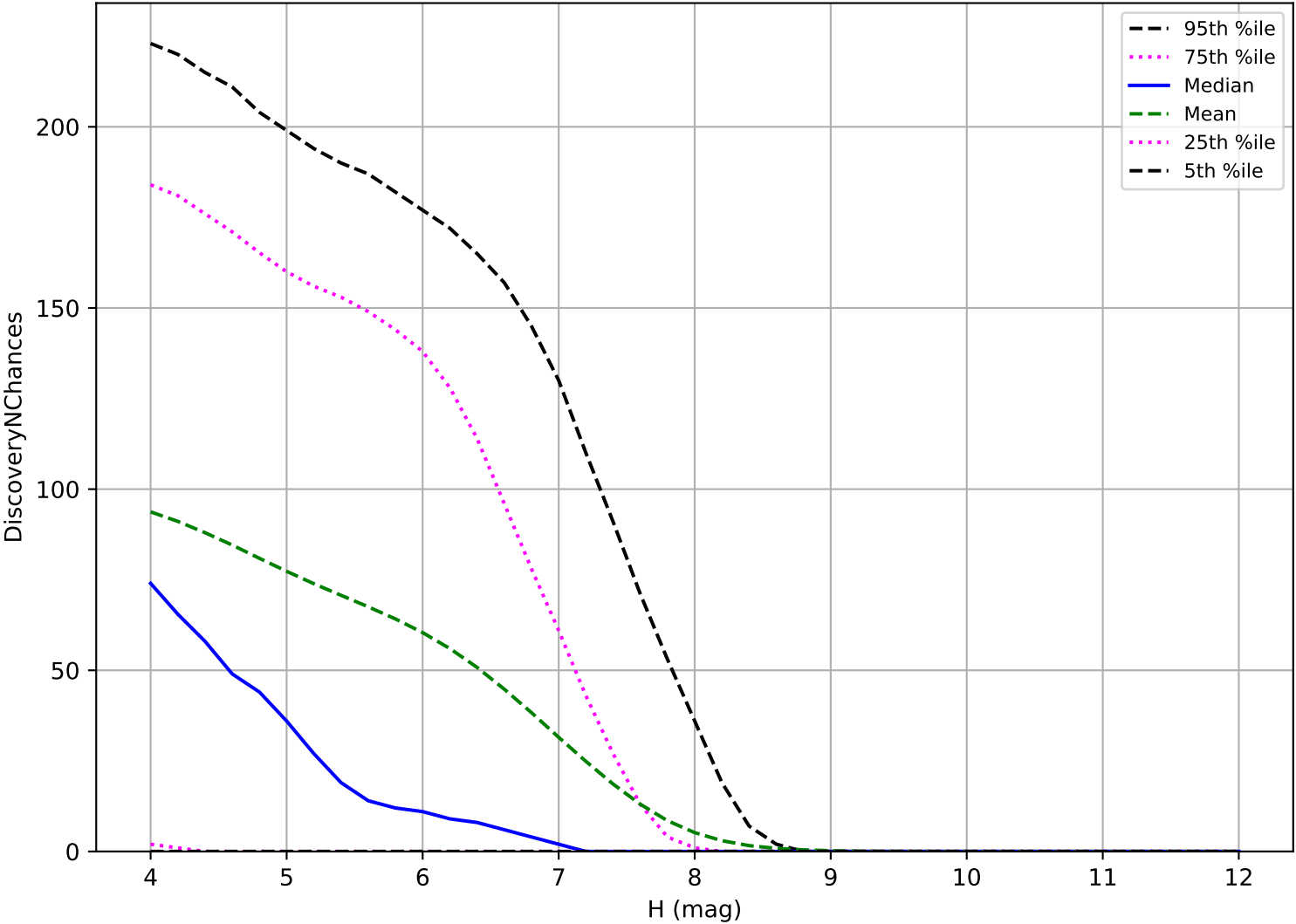
too_elab_heavy_r64_d3_ugrizy_v3.4_10yrs: TNO 3 pairs in 15 nights detection loss
