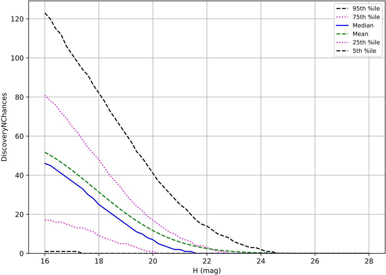
too_elab_heavy_r64_d3_ugrizy_v3.4_10yrs: PHA 3 pairs in 15 nights detection loss
