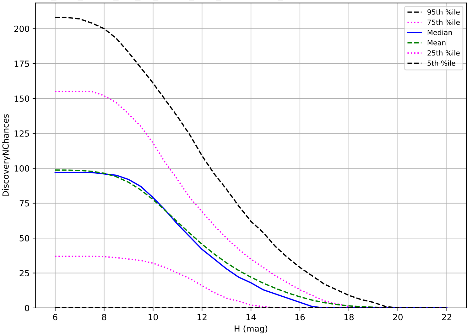
too_elab_heavy_r64_d3_ugrizy_v3.4_10yrs: OCC_r5 3 pairs in 15 nights detection loss
