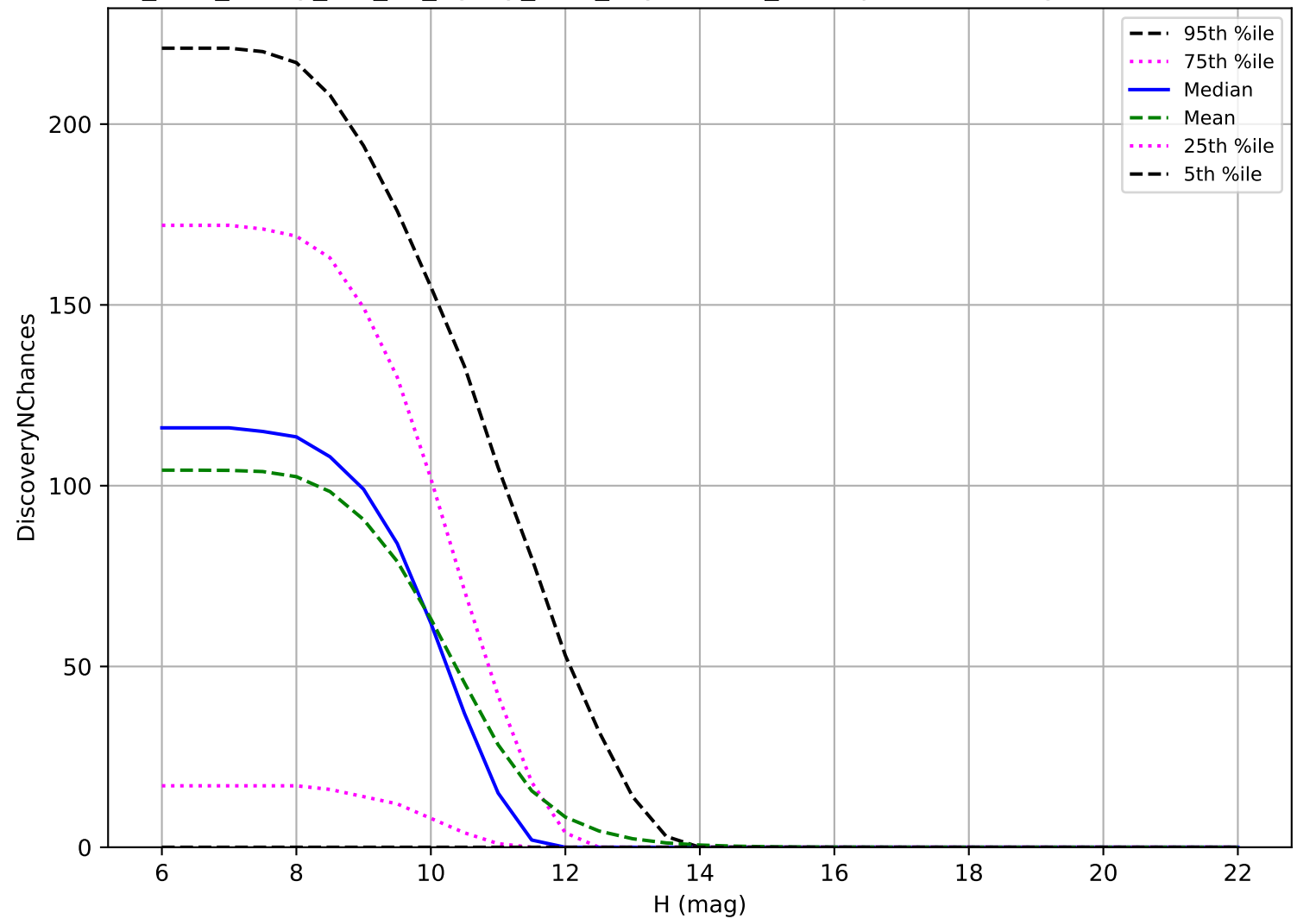
too_elab_heavy_r64_d3_ugrizy_v3.4_10yrs: OCC_r20 3 pairs in 15 nights detection loss
