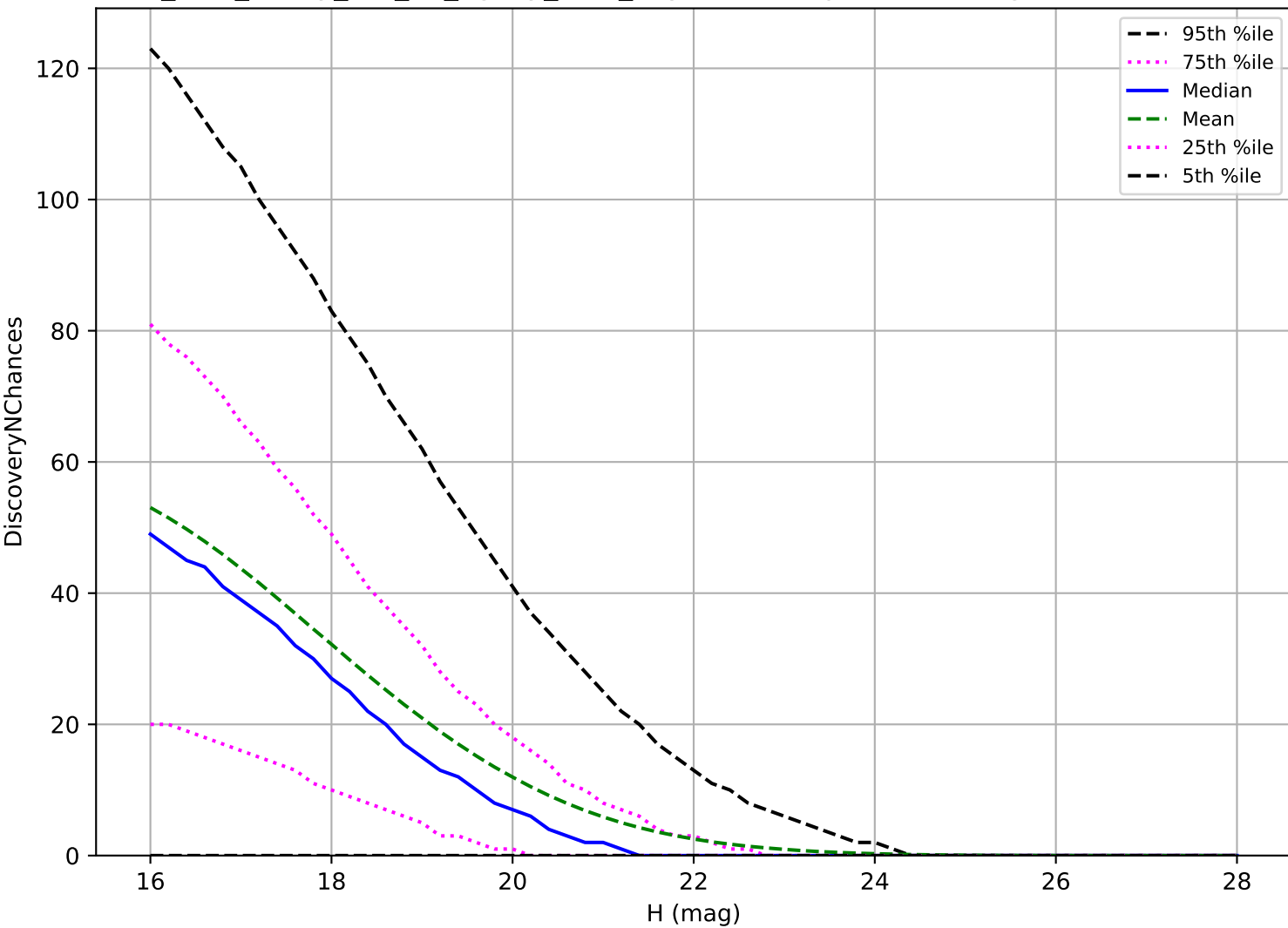
too_elab_heavy_r64_d3_ugrizy_v3.4_10yrs: NEO 3 pairs in 15 nights detection loss
