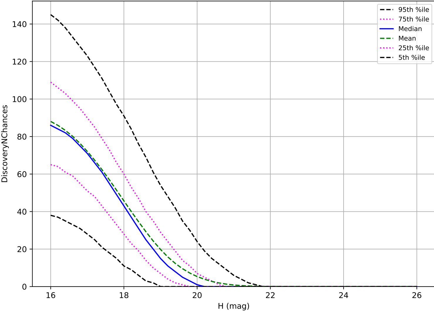
too_elab_heavy_r64_d3_ugrizy_v3.4_10yrs: MBA 3 pairs in 15 nights detection loss
