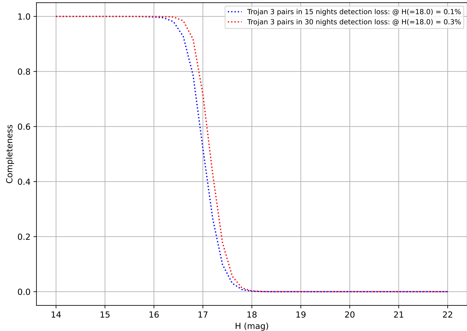
too_elab_heavy_r64_d3_ugrizy_v3.4_10yrs: DifferentialCompleteness
