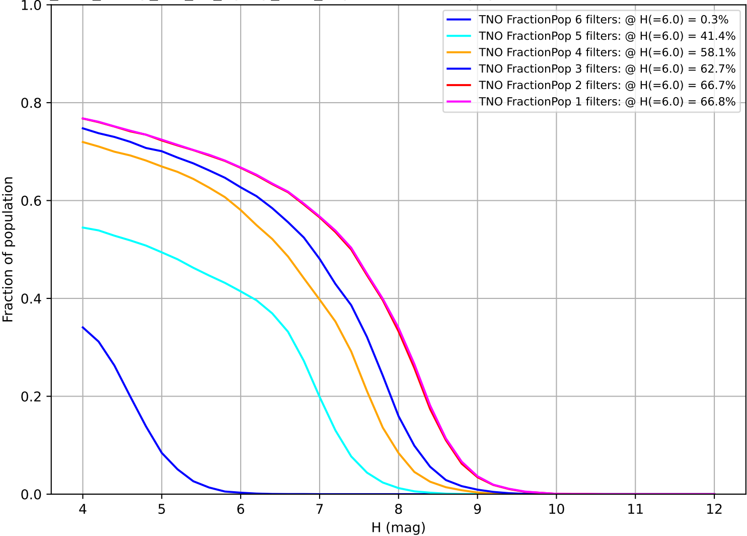
too_elab_heavy_r64_d3_ugrizy_v3.4_10yrs: Fraction of population with colors in X filters TNO
