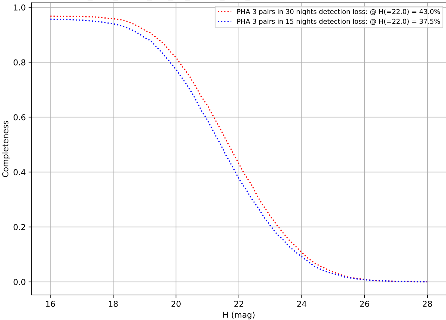
too_elab_heavy_r64_d3_ugrizy_v3.4_10yrs: DifferentialCompleteness
