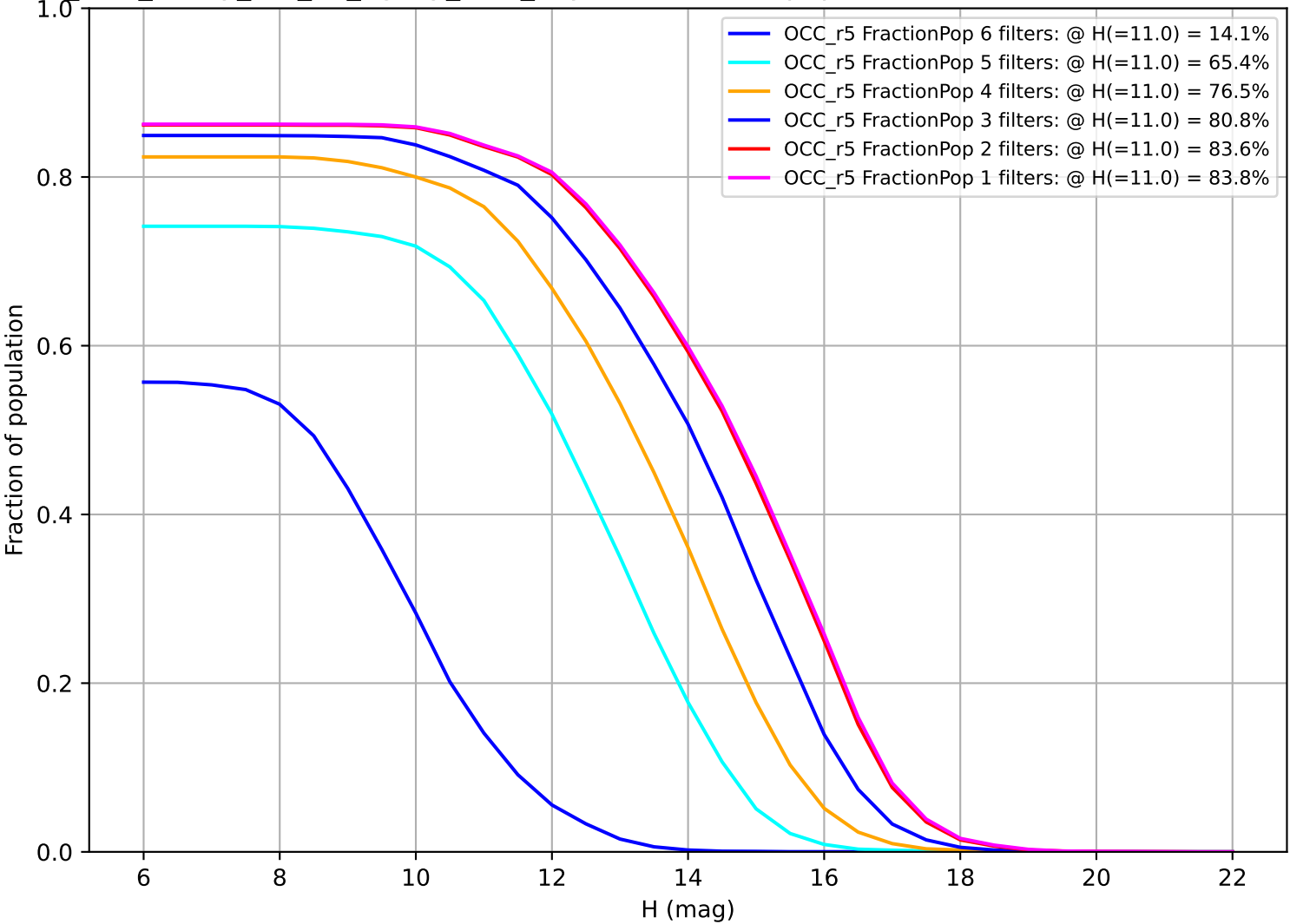
too_elab_heavy_r64_d3_ugrizy_v3.4_10yrs: Fraction of population with colors in X filters OCC_r5
