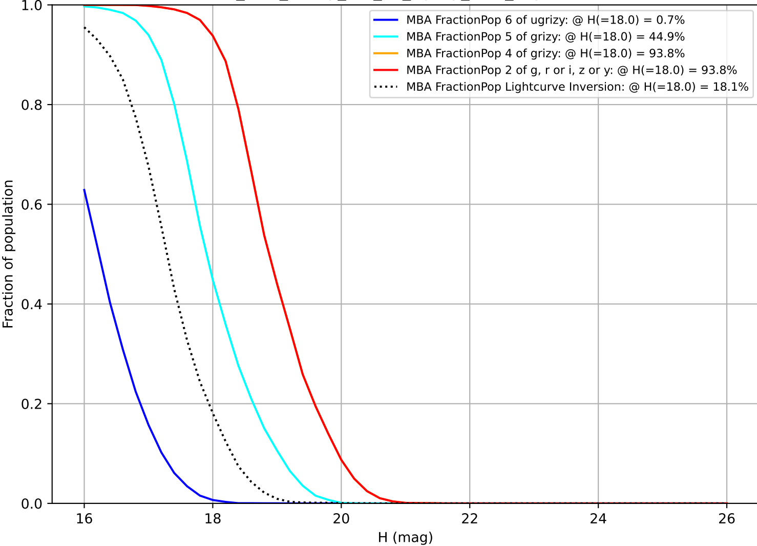
too_elab_heavy_r64_d3_ugrizy_v3.4_10yrs MBA
