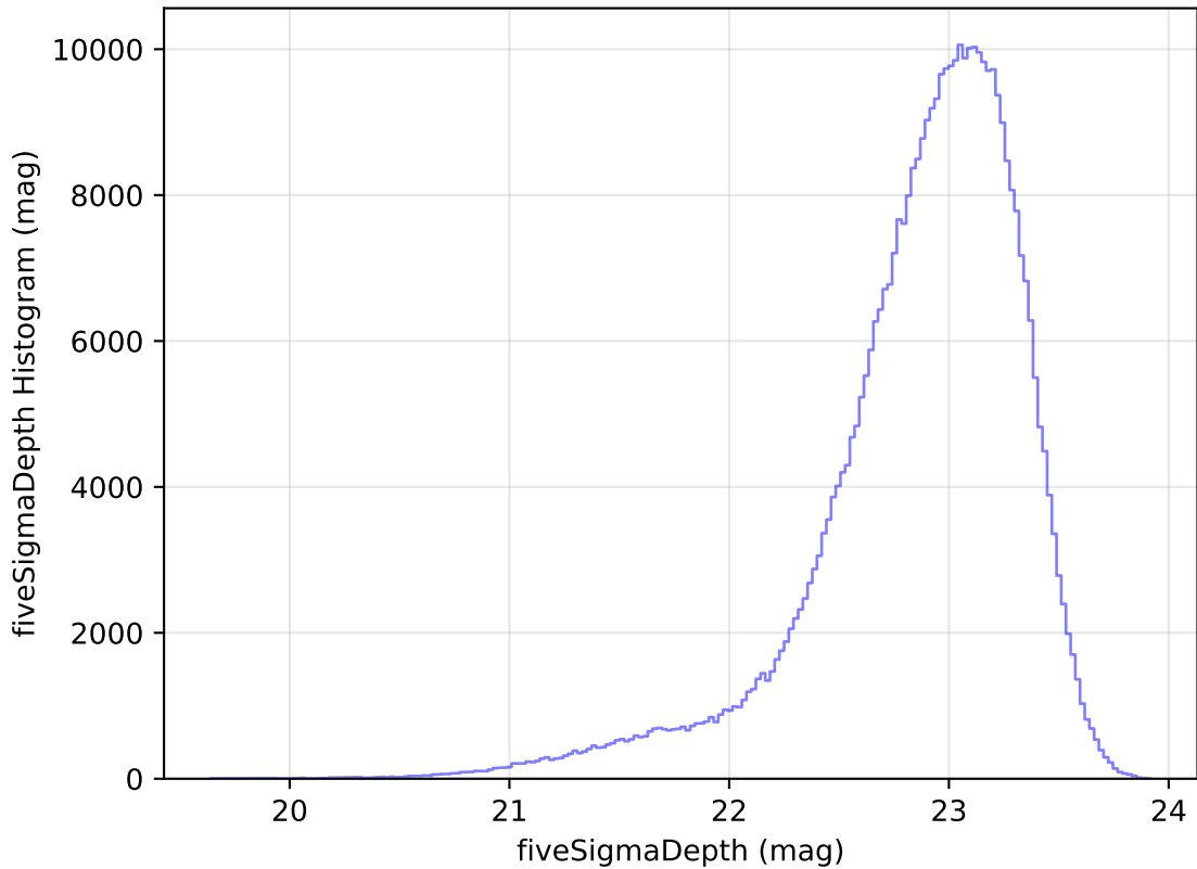
too_elab_heavy_r64_d3_ugrizy_v3.4_10yrs z: fiveSigmaDepth Histogram
