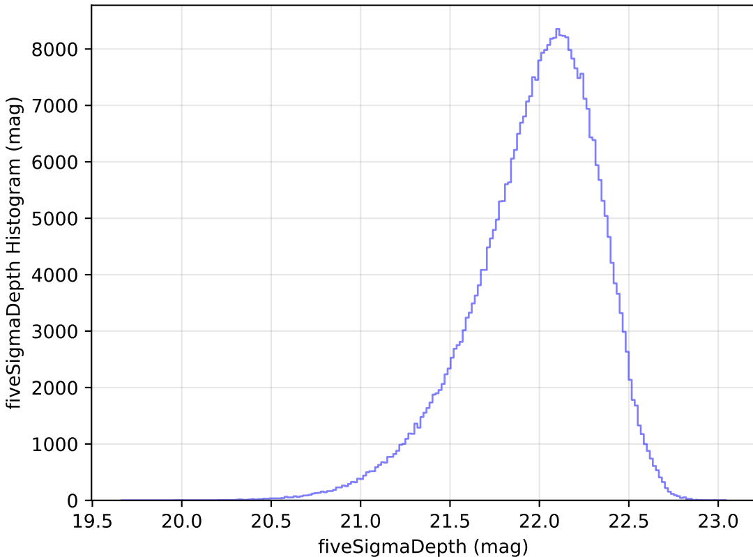
too_elab_heavy_r64_d3_ugrizy_v3.4_10yrs y: fiveSigmaDepth Histogram
