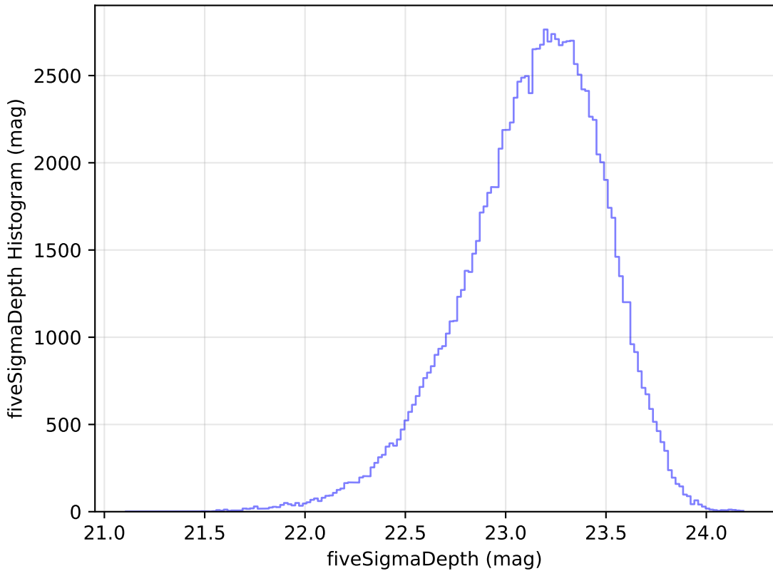
too_elab_heavy_r64_d3_ugrizy_v3.4_10yrs u: fiveSigmaDepth Histogram
