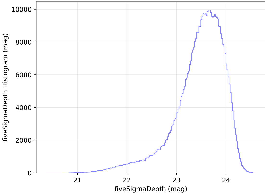
too_elab_heavy_r64_d3_ugrizy_v3.4_10yrs i: fiveSigmaDepth Histogram
