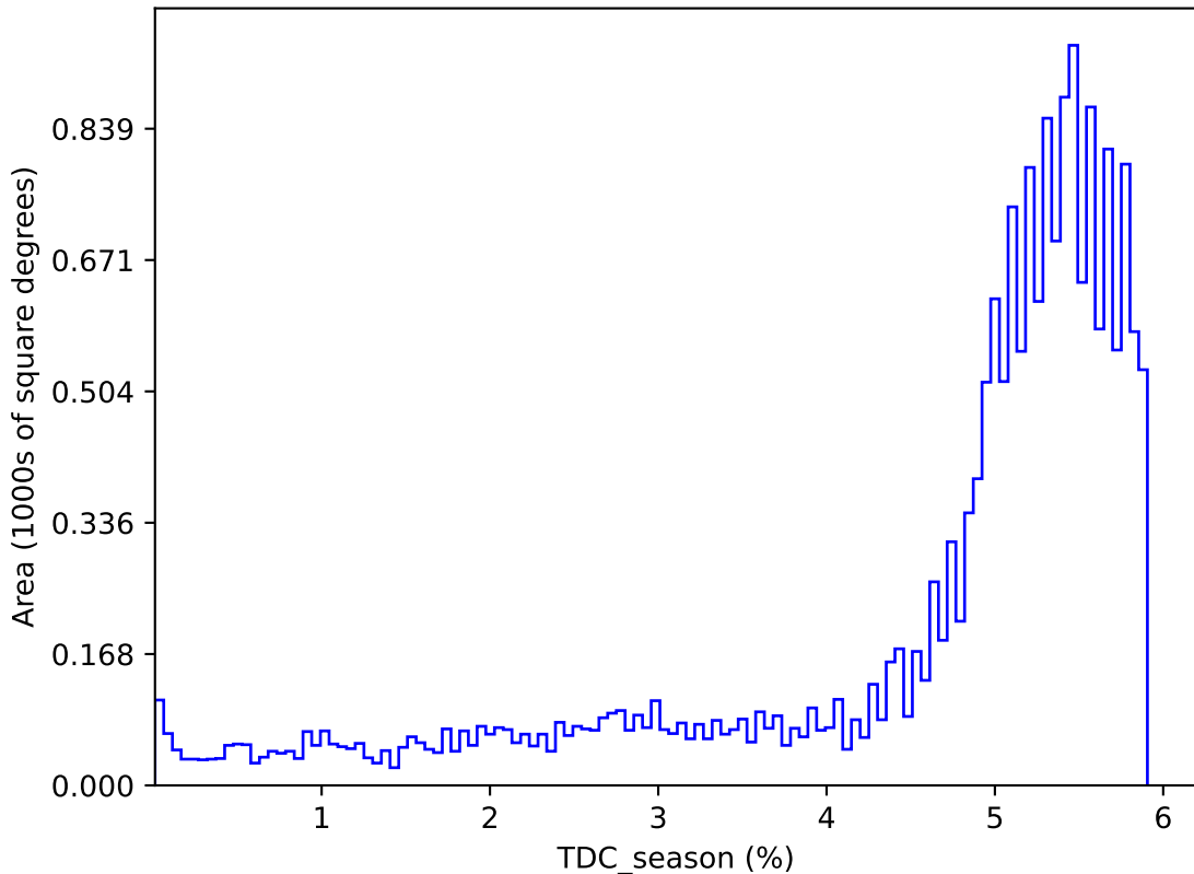
too_elab_heavy_r64_d3_ugrizy_v3.4_10yrs : TDC_season
