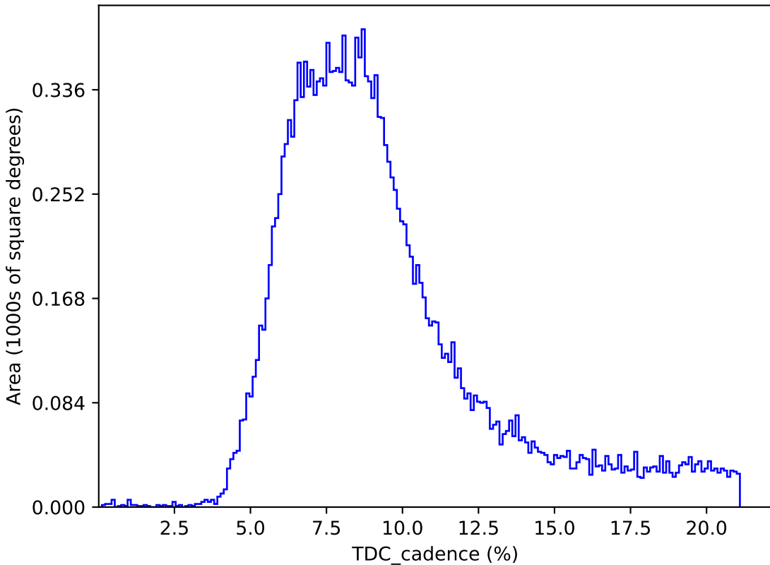
too_elab_heavy_r64_d3_ugrizy_v3.4_10yrs : TDC_cadence
