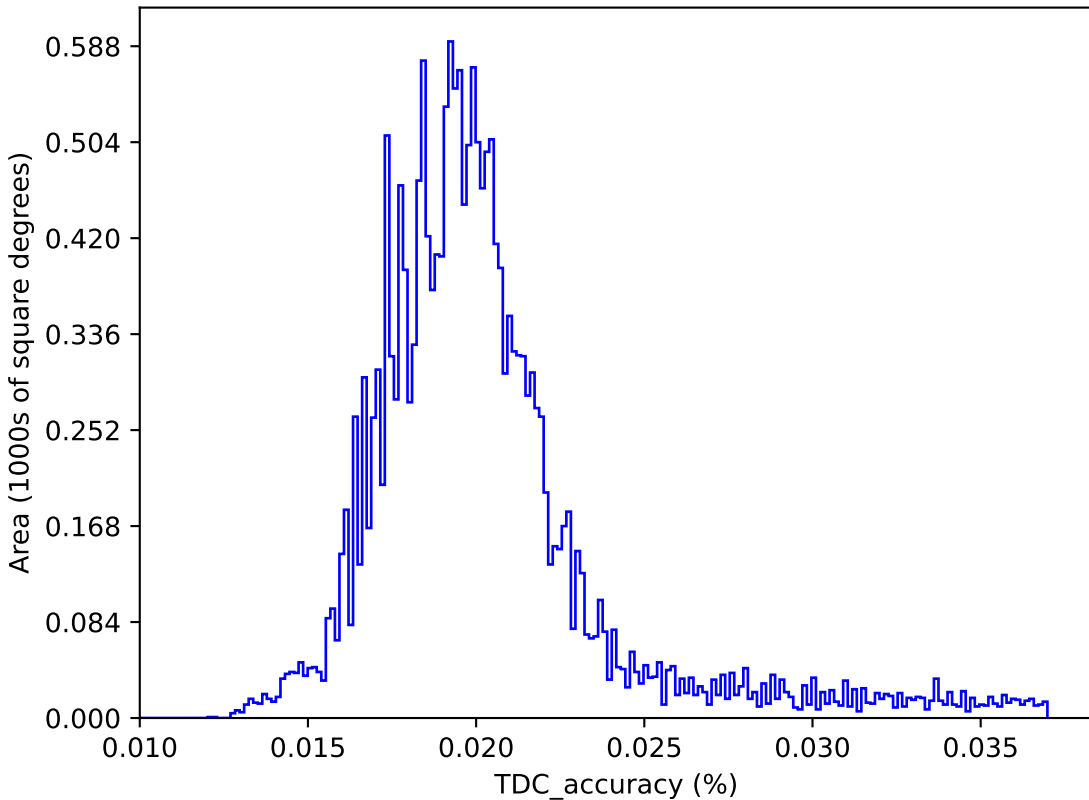
too_elab_heavy_r64_d3_ugrizy_v3.4_10yrs : TDC_accuracy
