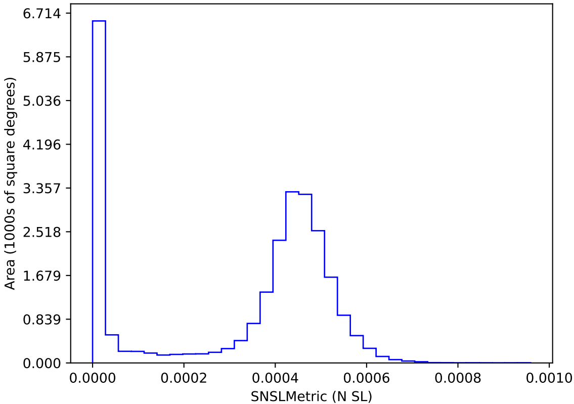
too_elab_heavy_r64_d3_ugrizy_v3.4_10yrs : SNSLMetric
