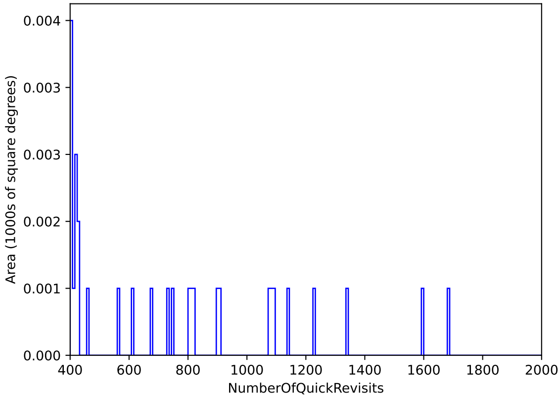
too_elab_heavy_r64_d3_ugrizy_v3.4_10yrs : NumberOfQuickRevisits
