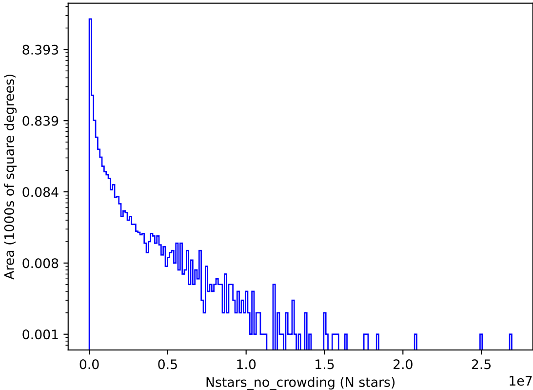
too_elab_heavy_r64_d3_ugrizy_v3.4_10yrs i: Nstars_no_crowding
